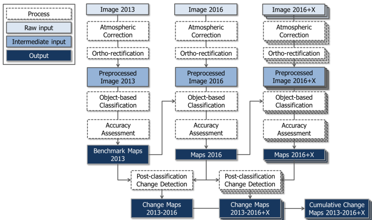
Figure 12: Schematic representation of the post-classification change detection process in order to analyse changes in mangrove and seagrass cover between the two time steps (2013, 2016). It is also illustrates how future post-classification change detections would be conducted and implemented.
