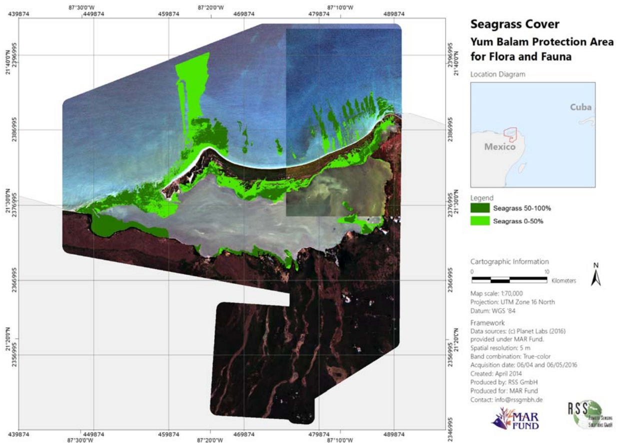
Figure 16: Seagrass cover classification for the Yum Balam Protection Area for Flora and Fauna for the year 2016. Shown are the two seagrass density classes (0-50%, and 50-100%). In the upper right diagram the location of the Yum Balam Protection Area for Flora and Fauna within Mexico is displayed (red).
